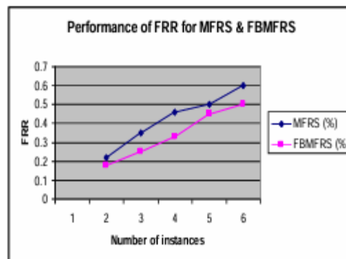
Fig 4. Performance of FRR for multimodal facerecognitionandfeaturebasedmultimodalfacerecognitionsystems.
