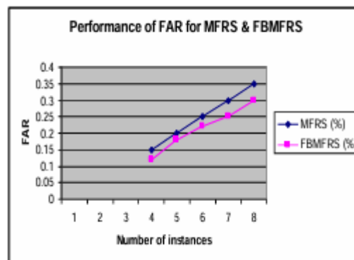
Fig 3. Performance of FAR for multimodal facerecognitionandfeaturebasedmultimodalfacerecognitionsystems.
